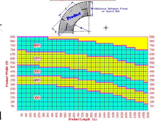
Conveyor Width Selection Chart 2
